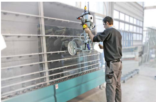
Vacuum lifting device VacuMaster Window for vertical handling of a glass sheet in a washing system
