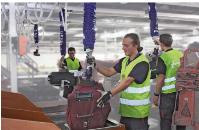
Vacuum tube lifter JumboFlex for handling baggage at airports
